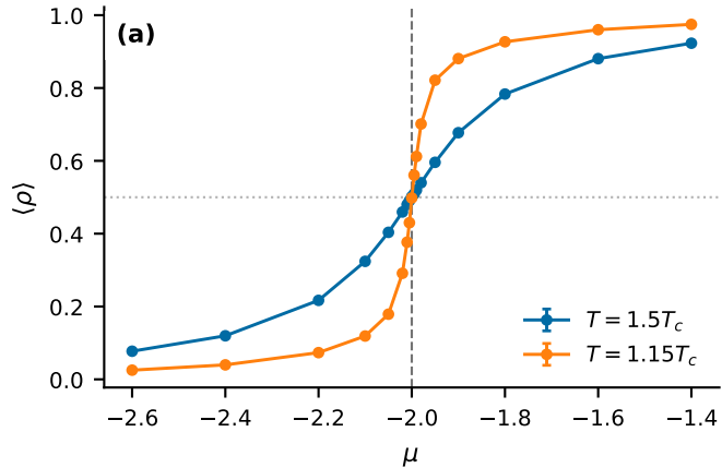
Equation of state
